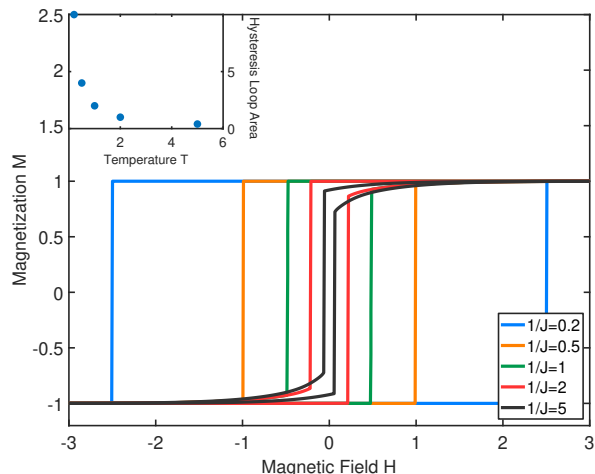
FIG. 7. Hysteresis loops at system size L = 64 , for different temperatures. The loops get narrower as temperature increases. The inset shows the loop area as a function of temperature. The loop area diverges as zero temperature is approached.
