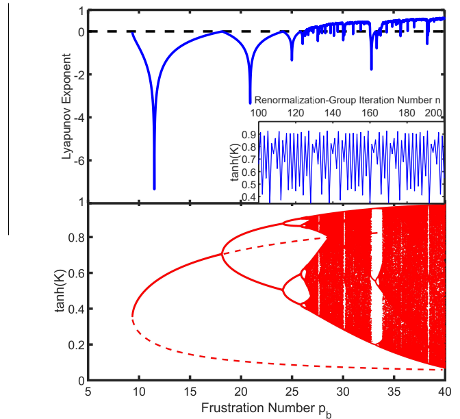
FIG. 2. Lower panel: The onset of chaos, by period doubling, under increased frustration for the q = 3 -state Potts model. For each p_b , the renormalization-group flows are in the vertical direction. The full lines represent attractive fixed points, limit cycles, and chaotic bands. The dashed lines represent the unstable fixed points, only some of which are shown. The \tanh(K) = 0 points are the stable fixed points which are the sinks of the disordered phase. The upper panel shows the calculated Lyapunov exponents. The upper inset shows the chaotic renormalization-group trajectory for p_b = 28 .
