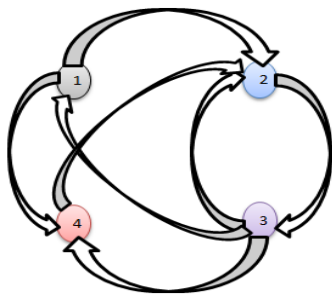
Figure 1. A graph with four nodes
