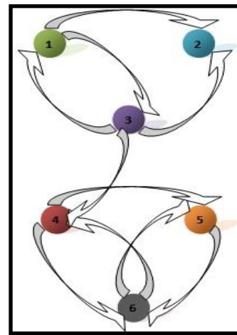
Figure 2. A graph with six nodes
