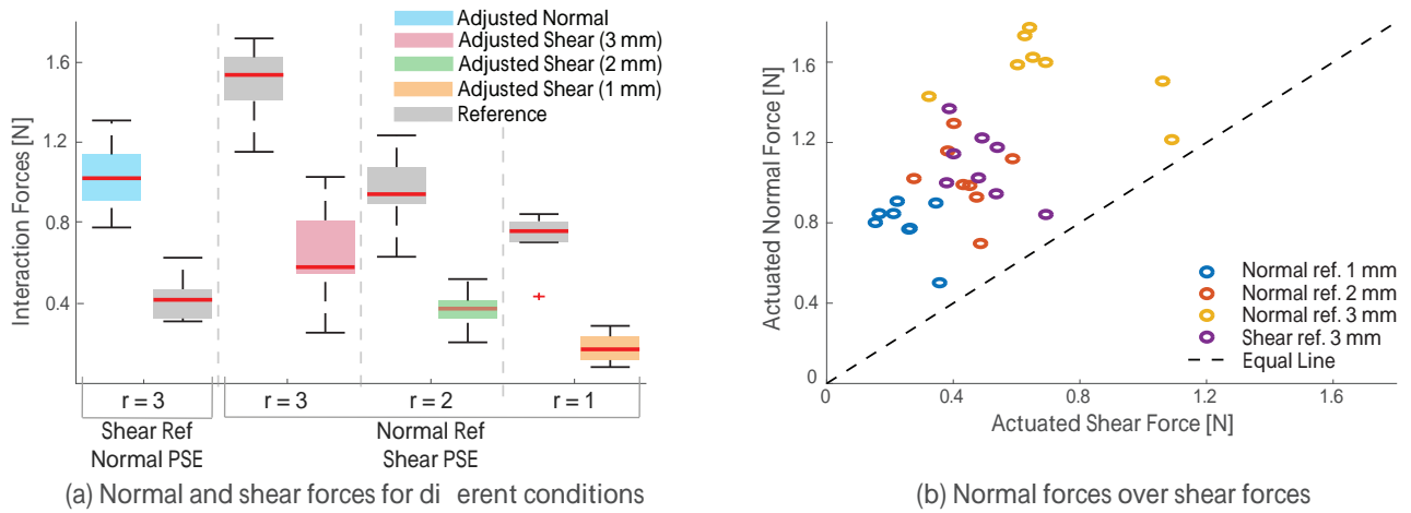
Fig. 9. Measured interaction forces for Experiment 2 when the normal reference is given as 1, 2, 3 mm and shear reference is given as 3 mm. ‘r’ represents the actuator displacement for the reference stimulus.
