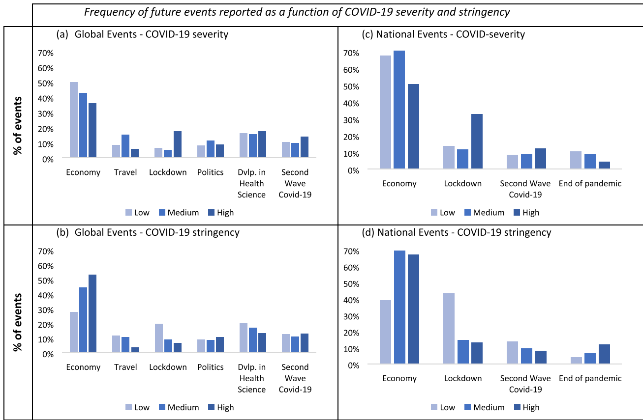
Fig. 2 Frequency of future events reported as a function of COVID-19 severity and stringency
