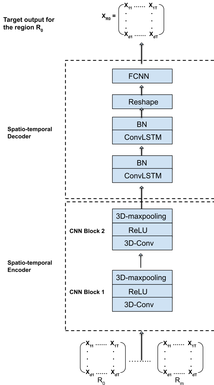
FIGURE 4. The proposed hybrid spatio-temporal autoencoder network architecture.
