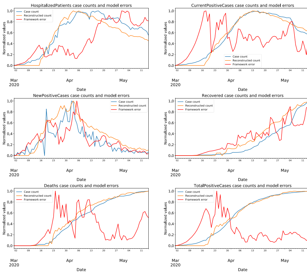
FIGURE 6. Model test results for the region Campania are given for features HospitalizedPatients, CurrentPositiveCases, NewPositiveCases, Recovered cases, Death cases, and TotalPositiveCases. Real case counts are plotted in blue, reconstructed case counts are plotted in orange, and reconstruction errors are plotted in red.
