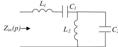
Figure 5. Obtained model for the dipole antenna.
